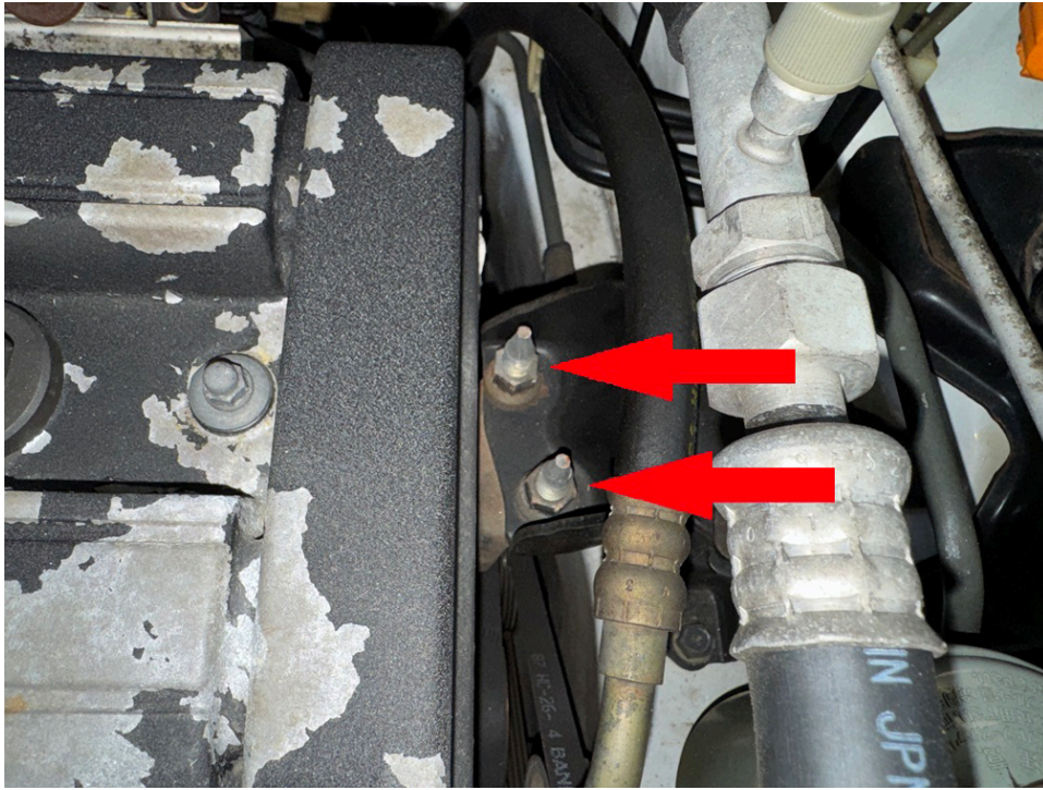
Step 6. Remove studs. Method 1: tighten 2 nuts against one another and back the stud out. Method 2. Weld nut to stud and back the stud out.
