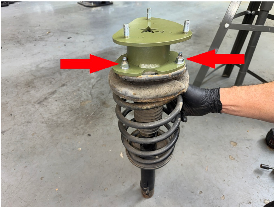
Step 37. Reinstall both driver and passenger side struts to shock tower using the OEM nuts. Torque nuts to 33 ft-lb.
