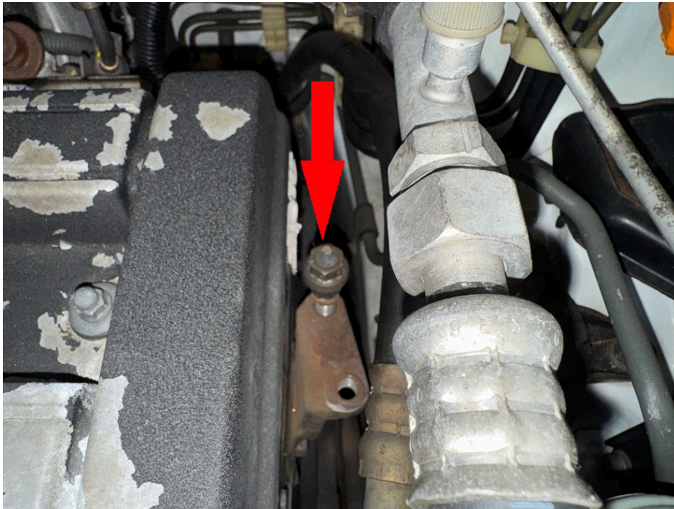
Step 7. Temporarily thread in M12x60 bolts included with the kit to keep engine in place when lowering subframe. Be sure to allow at least a 1.5 inch gap between engine and engine bracket.
