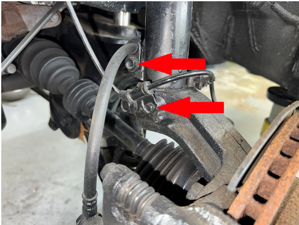
Step 28. Remove 17mm bolt holding strut to knuckle.
