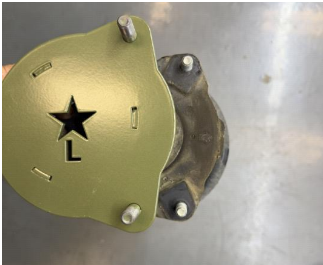
Step 9. Reinstall strut into shock tower with spacer attached, using original hardware. Spacer marked "L" is for DRIVER SIDE on U.S. models, spacer marked "R" is PASSENGER SIDE on U. S. models.
