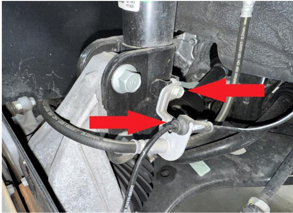
Step 5. Remove nuts connecting strut to knuckle. Tap bolts out with a hammer.
