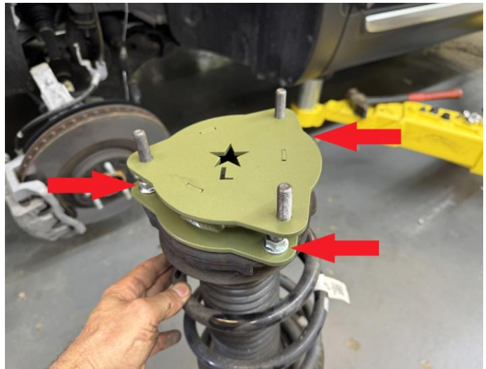
Step 9. Reinstall strut into shock tower with spacer attached, using original hardware. Spacer marked "L" is for DRIVER SIDE on U.S. models, spacer marked "R" is PASSENGER SIDE on U. S. models.
