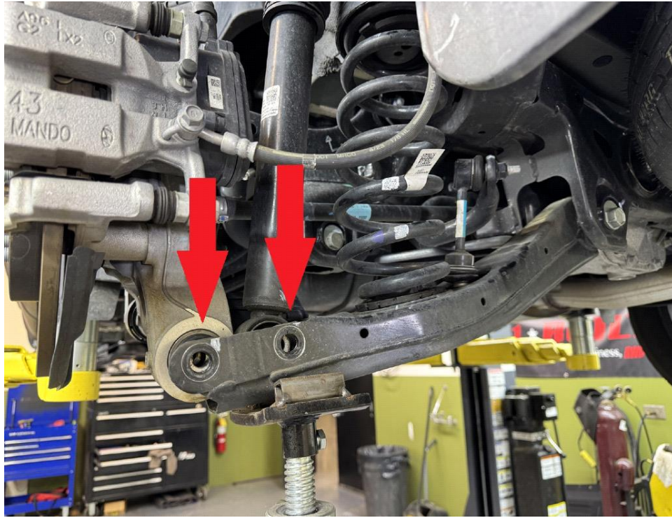
Step 20. Reinstall bolt holding shock to lower control arm.
