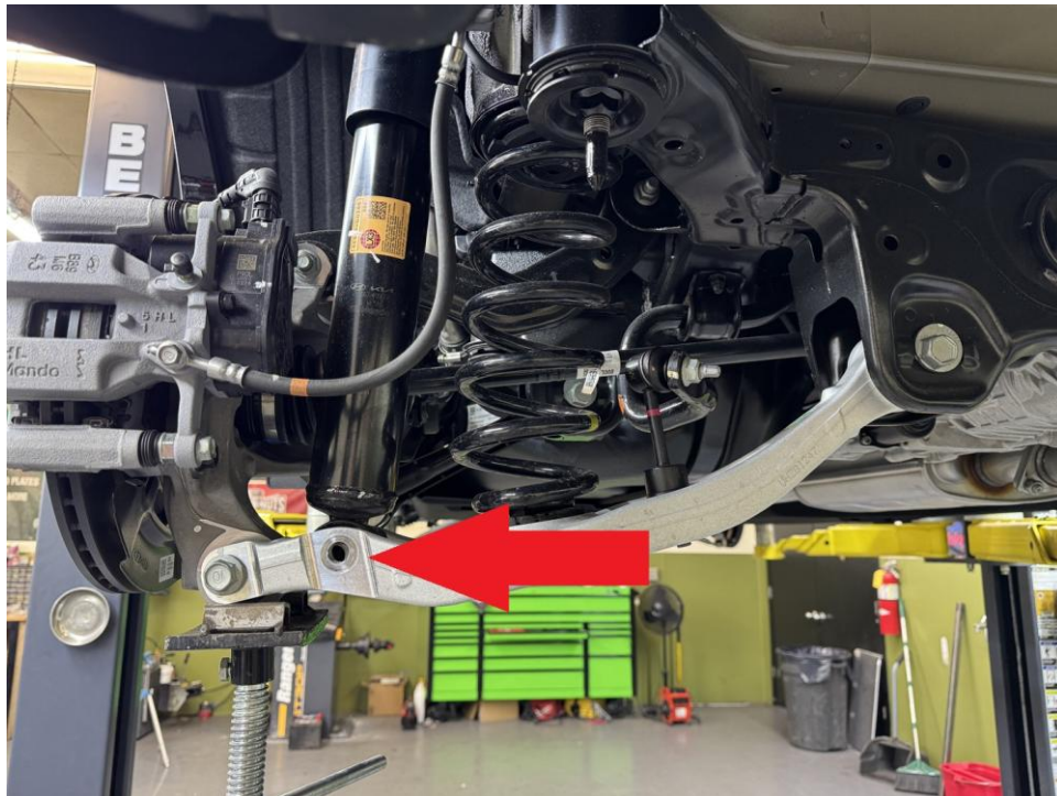
Step 21. Using a jack, lift lower control arm into position to line up bolt hole on wheel hub.
