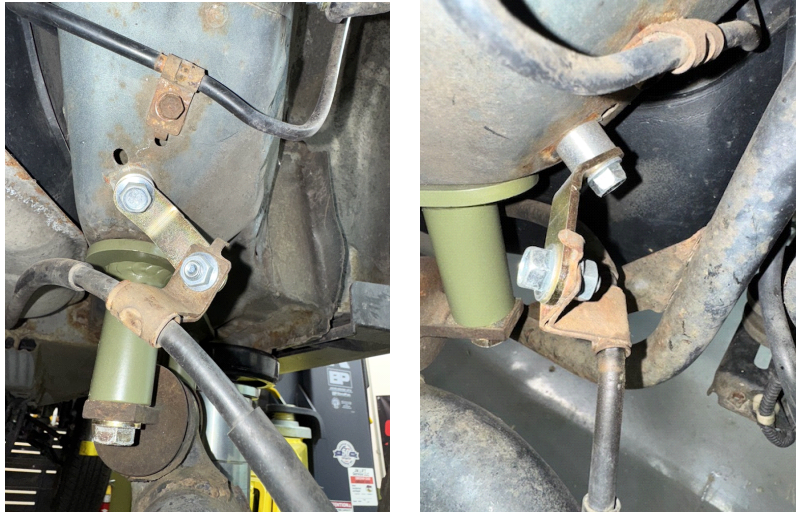
Step 27. Locate mount for rear brake line (lower) and install brake line bracket (lower) with M8 bolt and nut. (see photo)
