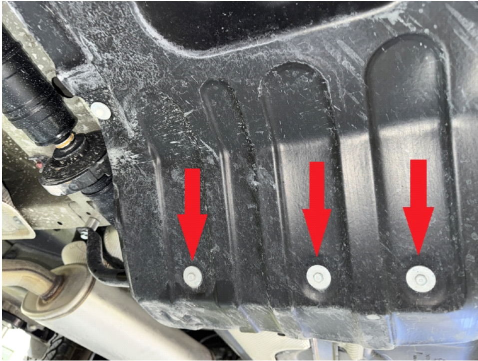
Step 13. Remove 3 12mm bolts holding gas tank bar to body.
