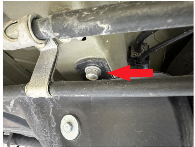
Step 14. Place 3 0.75x1.5 M8 spacers between gas tank bar and body, install 3 M8x60 bolts.
