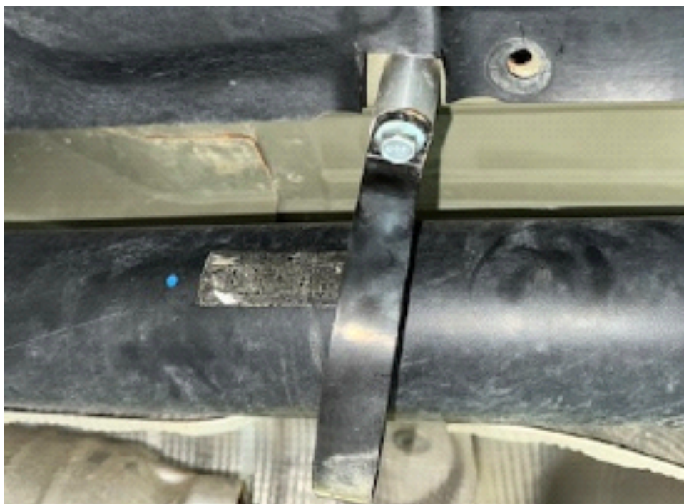
Step 8. Remove bolts holding driveshaft protector, place 0.75x1 M8 spacers between protector and body. (see photo)
