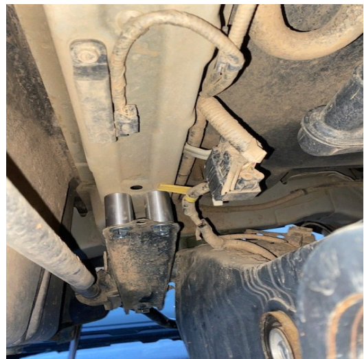
Step 8. Remove bolts holding driveshaft protector, place 0.75x1 M8 spacers between protector and body. (see photo)
