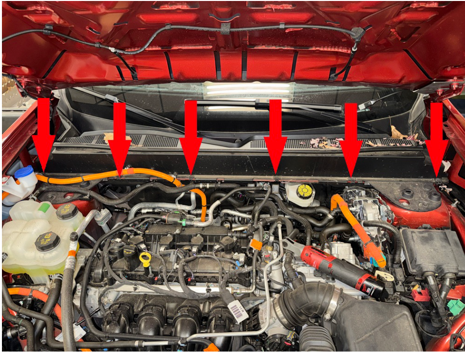
Step 8a ( HYBRID MODELS ONLY ) unclip wiring harness from cowl cover.
