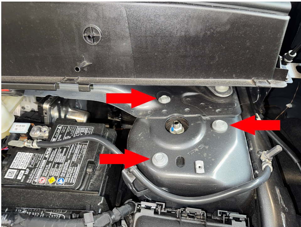
Step 11. Install lift spacer onto driver side strut using supplied M8x16 bolts as shown.
