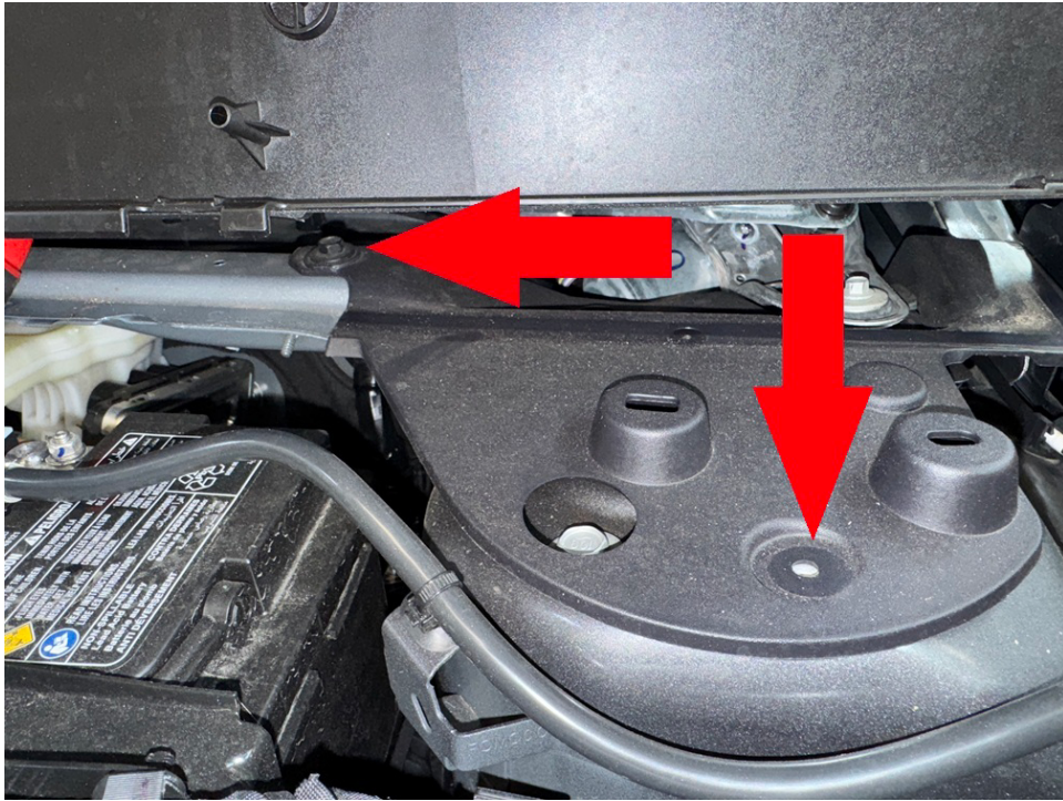
Step 10. Using a 13mm socket, remove the bolts at the top of the strut connecting strut to strut tower.
